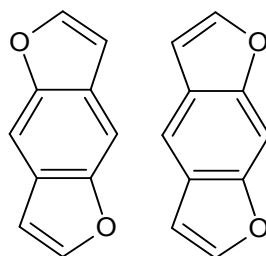
benzodifuranyl-
