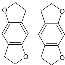
tetrahydrobenzodifuranyl-
